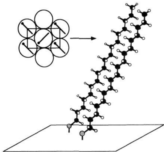
Figure 15. Illustration of the structure of a monolayer of an octadecanethiolate monolayer on gold inferred from a two-chain simulation based on all-trans chains. The inset shows the relationship of an orthorhombic chain sublattice (uncanted) relative to the hexagonal sulfur sublattice and the direction of the cant of the hydrocarbon chain for this arrangement as inferred from IR spectroscopy.
