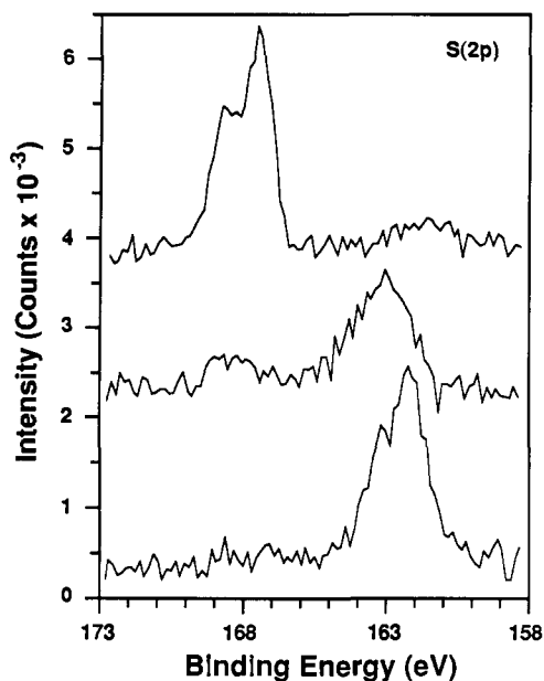
Figure 12. Effect of exposure to atmosphere on XPS spectra of octadecanethiolate monolayers on copper (bottom, <1 h; middle, ~2 wk). The upper spectrum is of a silver surface derivatized in an iso-octane solution of hexadecanesulfonic acid, presumably adsorbed as the sulfonate anion, and is provided for comparison. All spectra (40 scans) were referenced to C(1s) = 284.80 eV. The lower spectrum exhibits a S(2p) envelope consistent with a thiolate attachment; the sample exposed to atmosphere for 2 weeks displays peaks associated with the partial attachment of the monolayer via a sulfonate moiety (see Table I) and confirms assignments in Figure 11. XPS was less sensitive to the presence of oxidized head groups that IR; longer exposures to atmosphere were required to confirm the products of oxidation by XPS. Similar changes are observed in the S(2p) spectra of alkanethiolate monolayers on silver although they occur at a slower rate.
