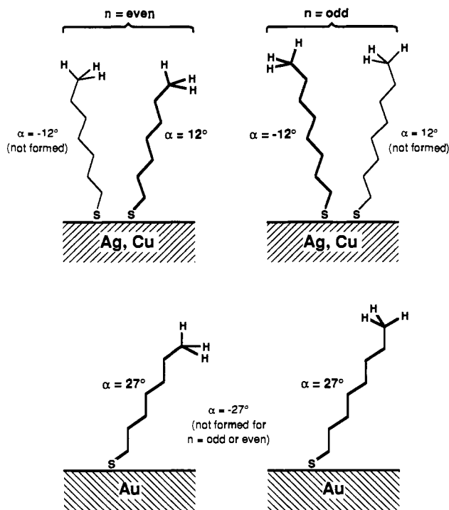
Figure 14. Illustration of the canted structures formed upon adsorption of n -alkanethiols, \text{CH}_3(\text{CH}_2)_n\text{SH} , on copper, silver, and gold. The structures that form on copper and silver do not exhibit any change in the intensities of methyl modes with incremental increase in the number of methylene groups (Figures 4 and 5). This observation is consistent only with the formation of a structure in which the cant angle, \alpha , is positive for an even number of methylene groups and negative for an odd number of methylene groups; the geometry of the metal-thiolate interaction on these metals is not fixed as n is varied (upper panel). The structures formed on gold exhibit an odd-even modulation in the intensities of the methyl modes with increasing chain length (Figures 4 and 5). This modulation reflects the formation of a structure in which variations in the chain length of the adsorbate do not perturb the geometry of the gold-thiolate interaction (lower panel).
